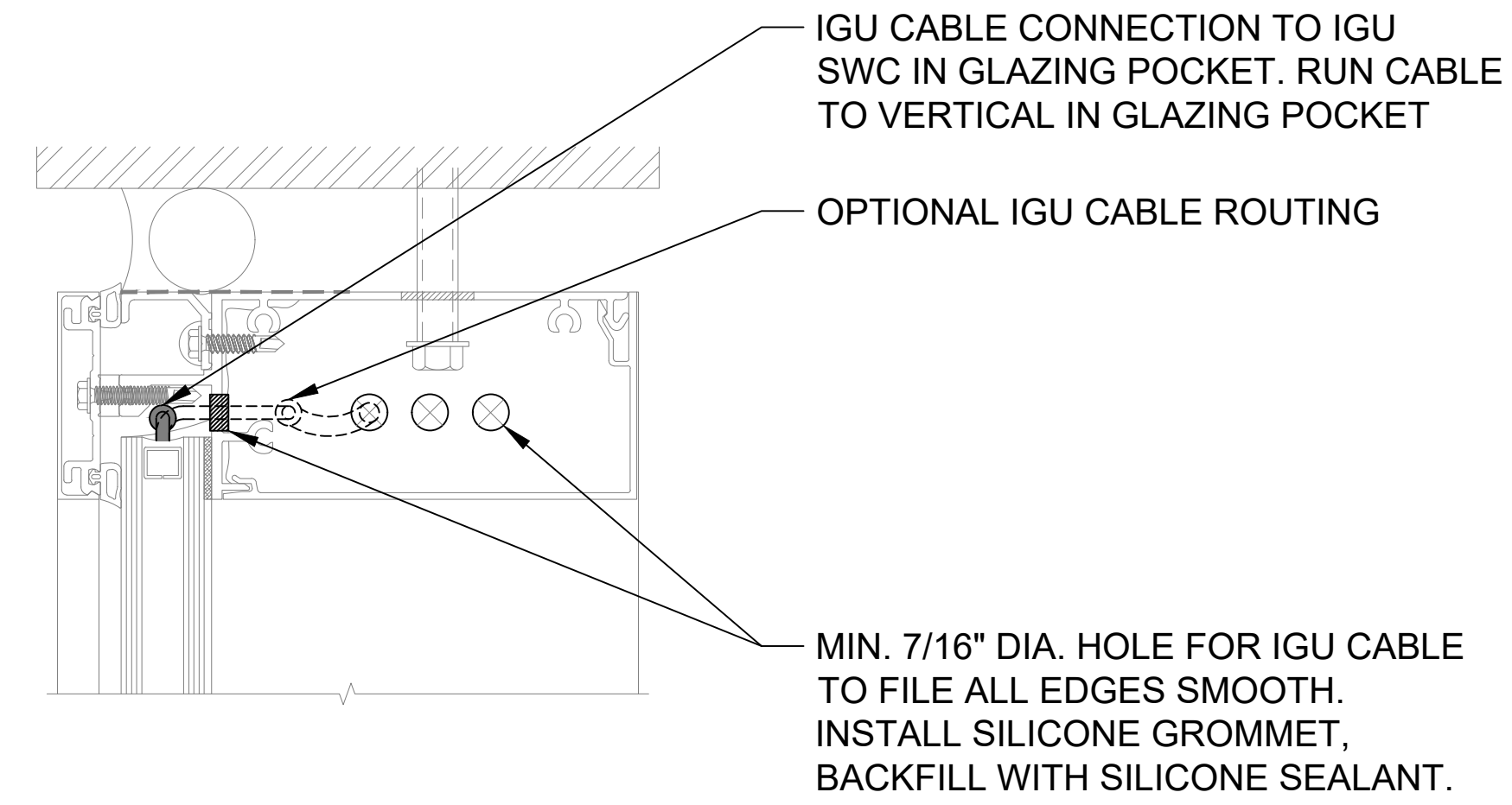
DETAIL 1 HEAD
