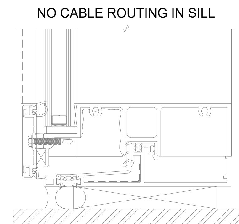
DETAIL 3 SILL
