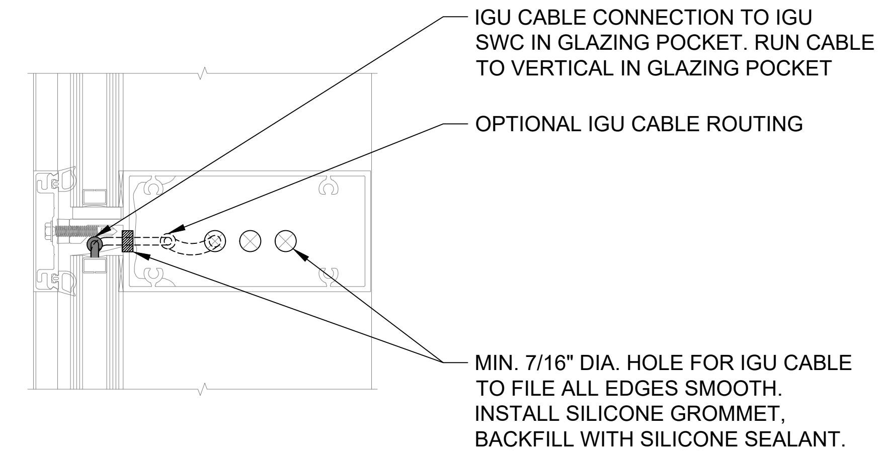
DETAIL 2 HORIZONTAL MULLION
